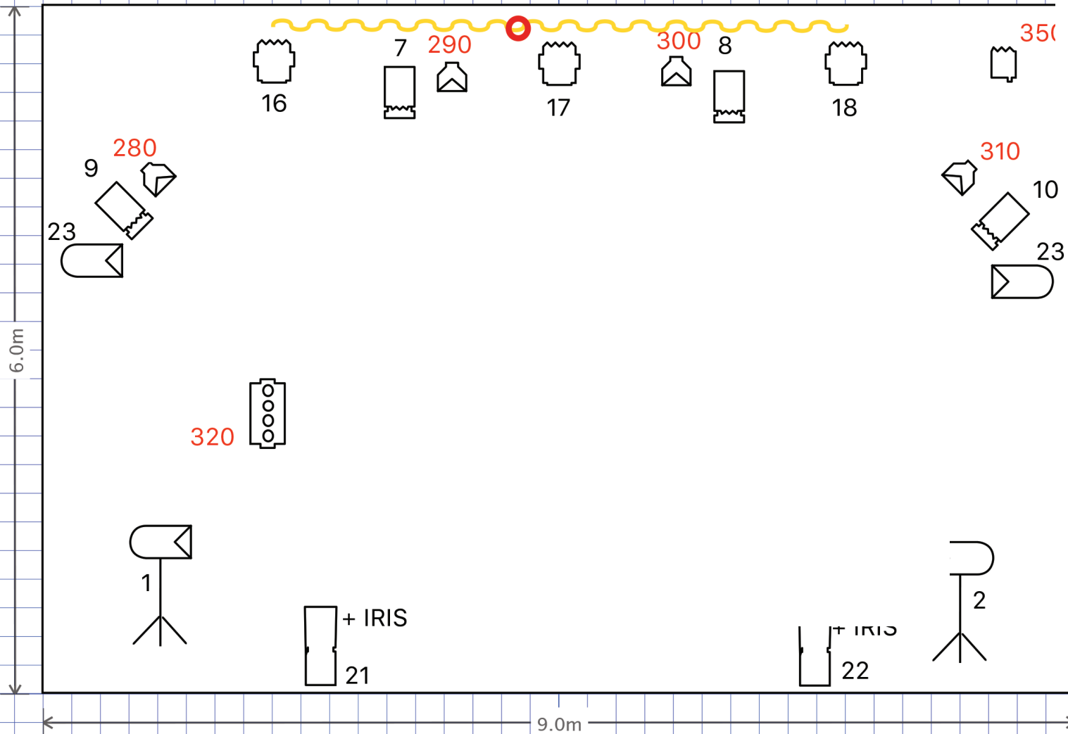
Plan Sol
